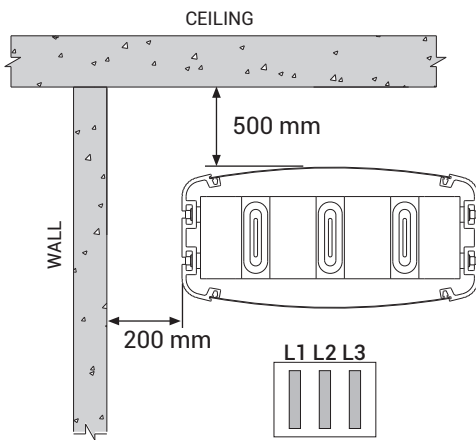
FIGURE 1 - EDGEWISE APPLICATION
